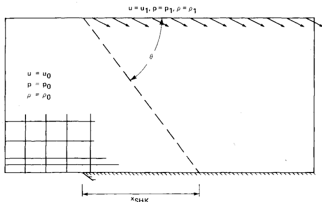
Fig. 2 Initial flowfield for shock/boundary-layer interaction.
