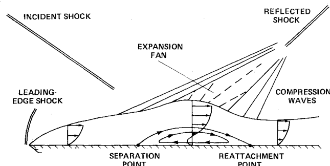
Fig. 1 Sketch of shock/boundary-layer interaction.
